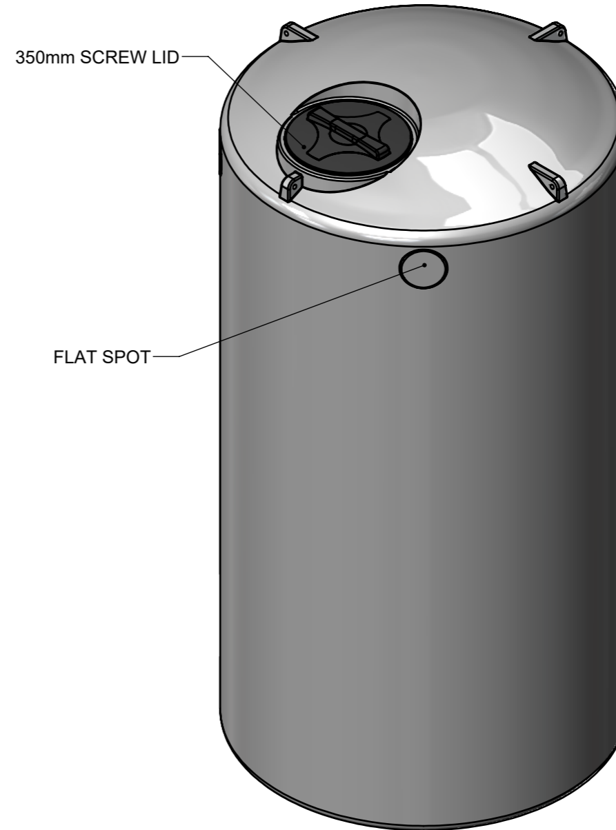
PICTORIAL VIEW
