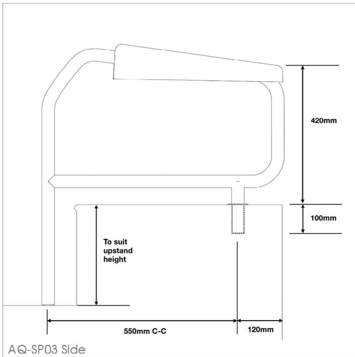
AQ-SP03-B with White Top and Numbered
